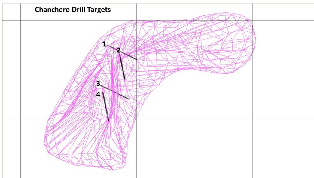
Figure 1: Locations of 4 Proposed drill holes at the Chanchoero target, relative to the outline/projected shape of the greater at than 50MV/V chargeability anomaly as defined by the 2008 3-D Induced Polarization survey.
